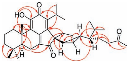
Figure 1. Key HMBC correlations of compound 1 .
